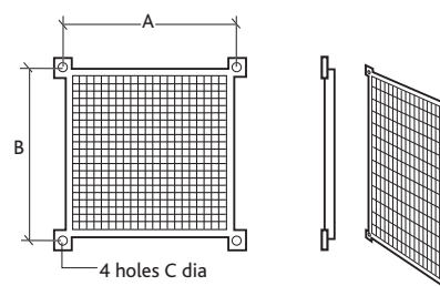
Figure 1. End view of recommended vertically mounted unit installation (bracket supplied).
