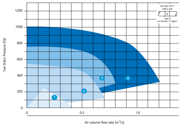
Xtractor Internally Mounted Fan Units 1-4
