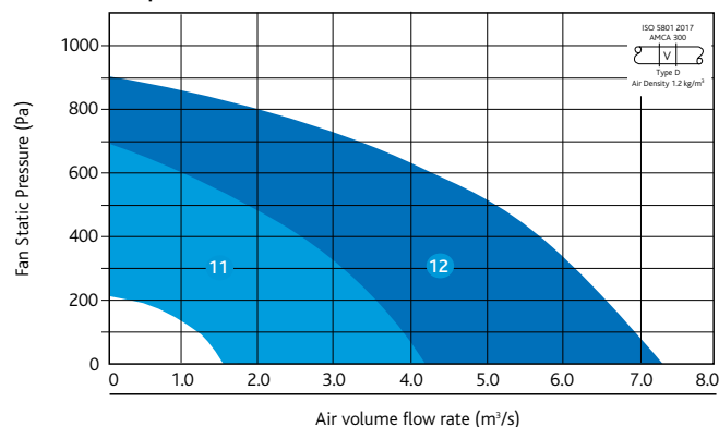
Airmover - 6 pole
