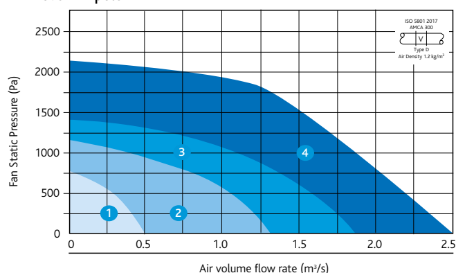
Airmover - 2 pole
