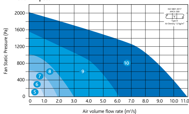
Airmover - 4 pole
