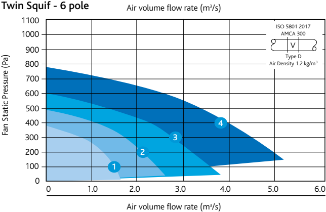
Twin Squif - 6 pole
