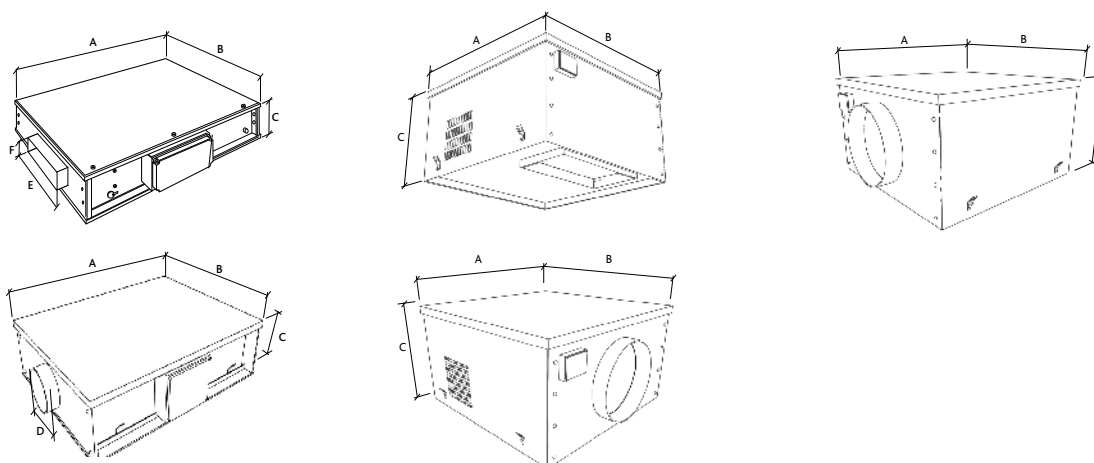
DIMENSIONS (MM)
