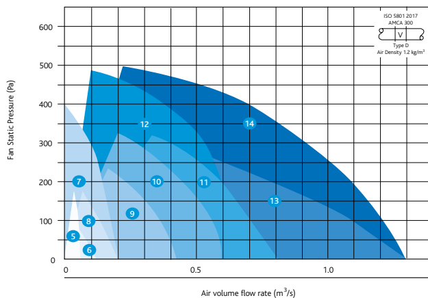
Xtractor Internally Mounted Fan Units 5-14
