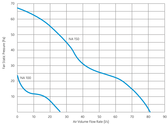
NA100 & 150 Single Speed Fans
