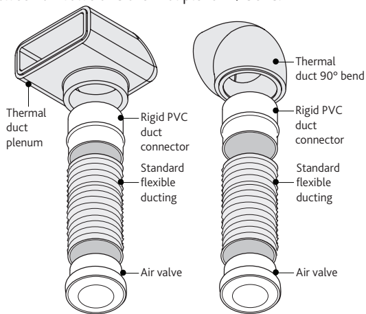
4 Typical semi rigid acoustic flexible duct connection between air valve and thermal plenum / bend.
