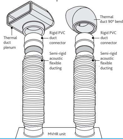
3 Typical semi rigid acoustic flexible duct connection between MVHR and thermal plenum / bend.
