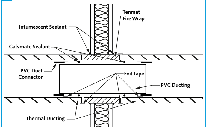
7 Typical fire wrap installation using PVC duct connections.
