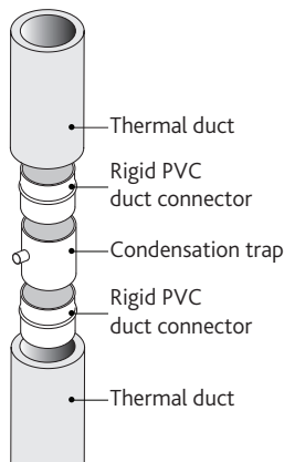
5 Condensate trap with rigid PVC duct connectors.
