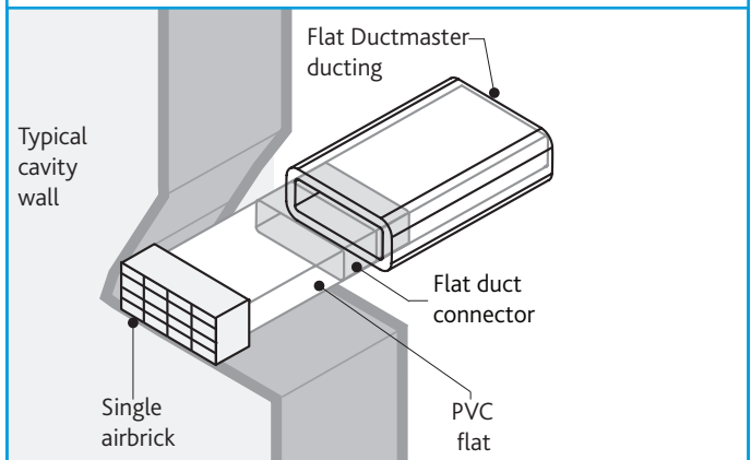
6 Typical rectangular thermal duct connection to air brick.
