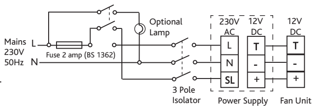
Figure 4b. Wiring. PCB details
