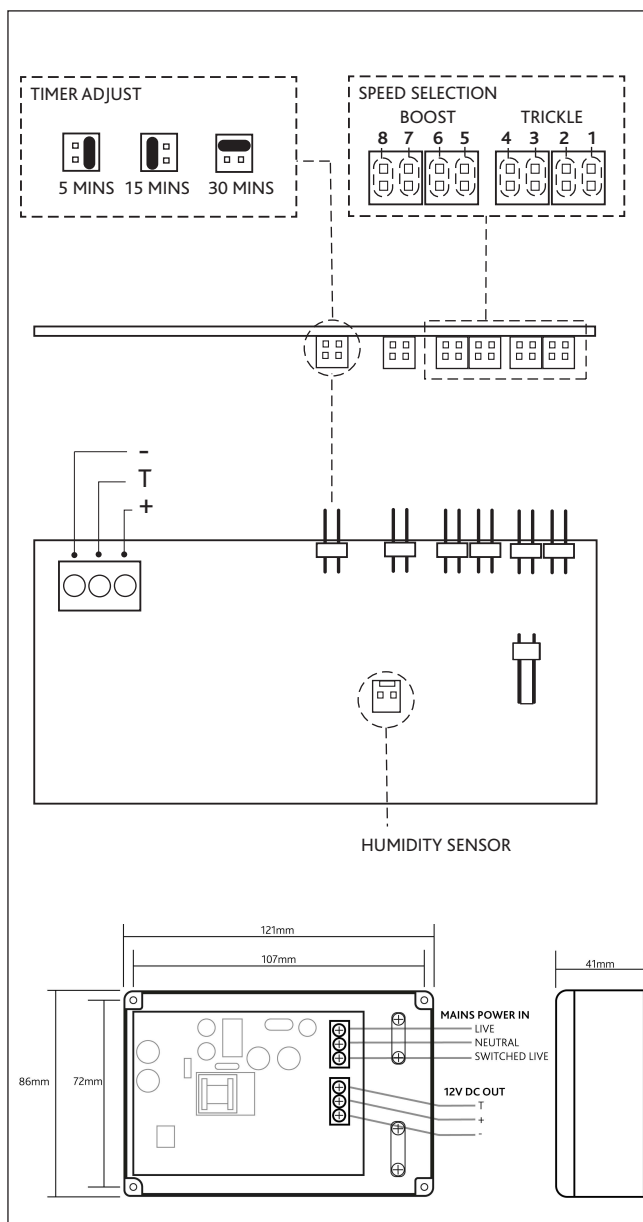
Figure 4b. Wiring. PCB details
