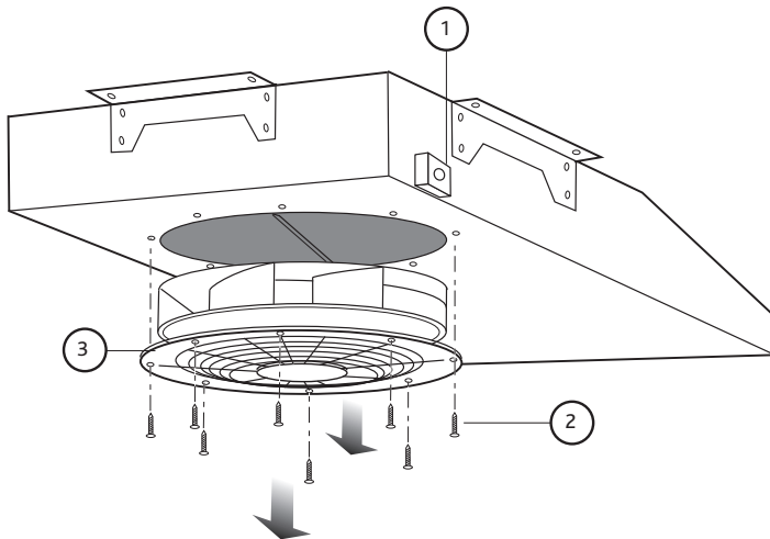
Figure 5. Impeller removal and dismantling.
