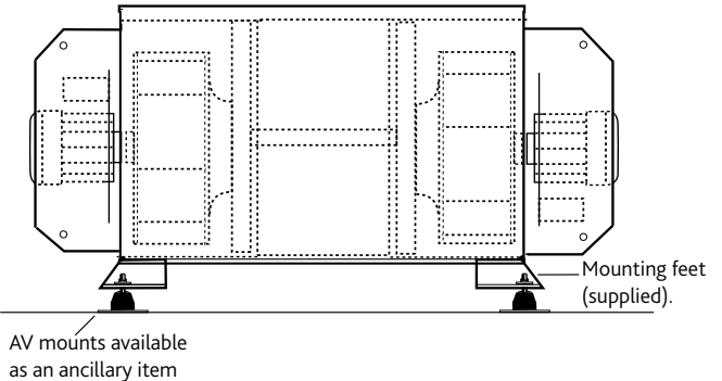
Figure 1. AV mounts fitted to unit mounting feet (supplied) in horizontal discharge mode.
