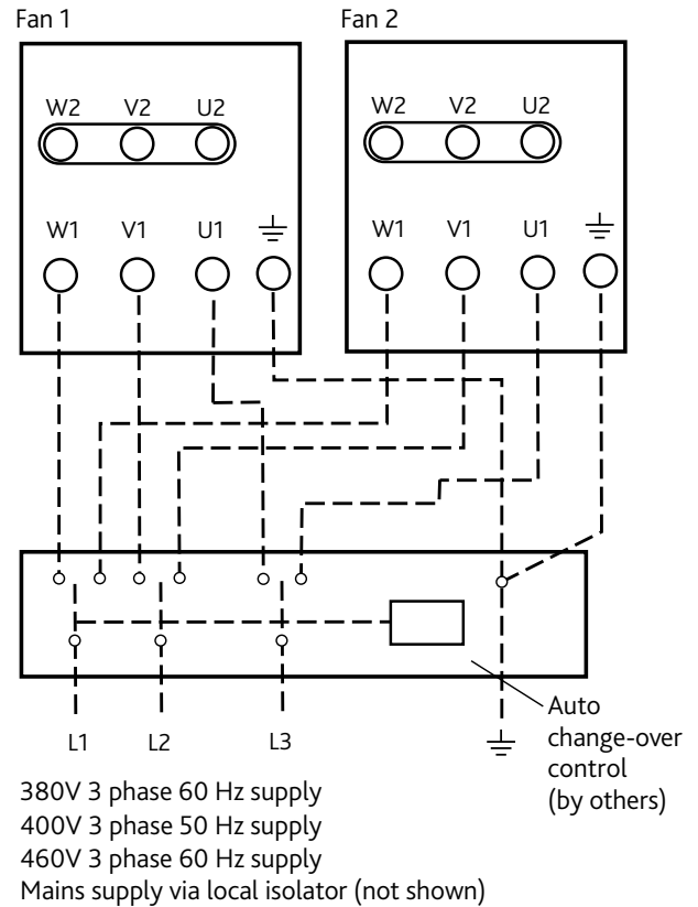
Figure 5. Three phase fans Single speed - motors up to 3kW inclusive.
