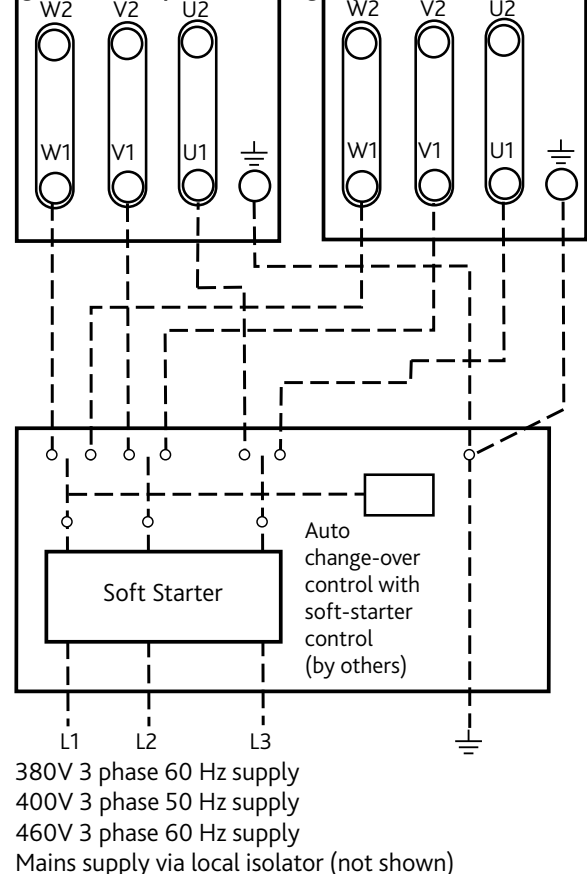
Figure 6. Three phase fans Single speed - motors 4kW or above.
