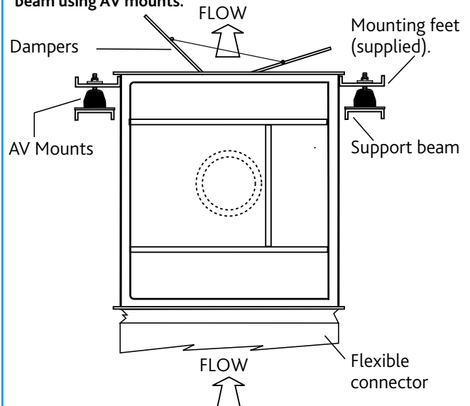
Figure 2. Unit in vertical discharge mode, mounted on support beam using AV mounts.
