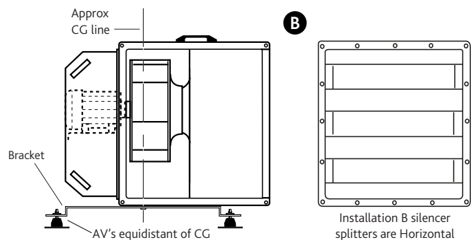
Figure 3. End view of non-recommended horizontally mounted unit installation (bracket by others).
