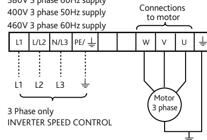
Figure 9. 3 phase units with matched frequency inverter single speed.
