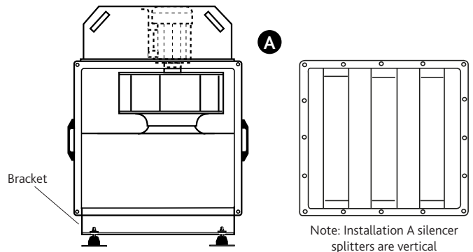
Figure 2. End view of recommended vertically mounted unit installation (bracket supplied).
