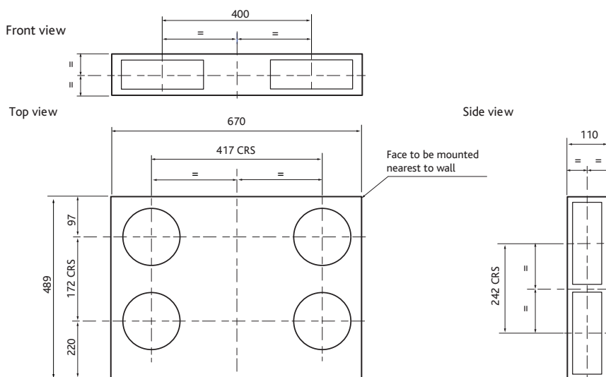
Figure 11. MRXBOX-FF2.
