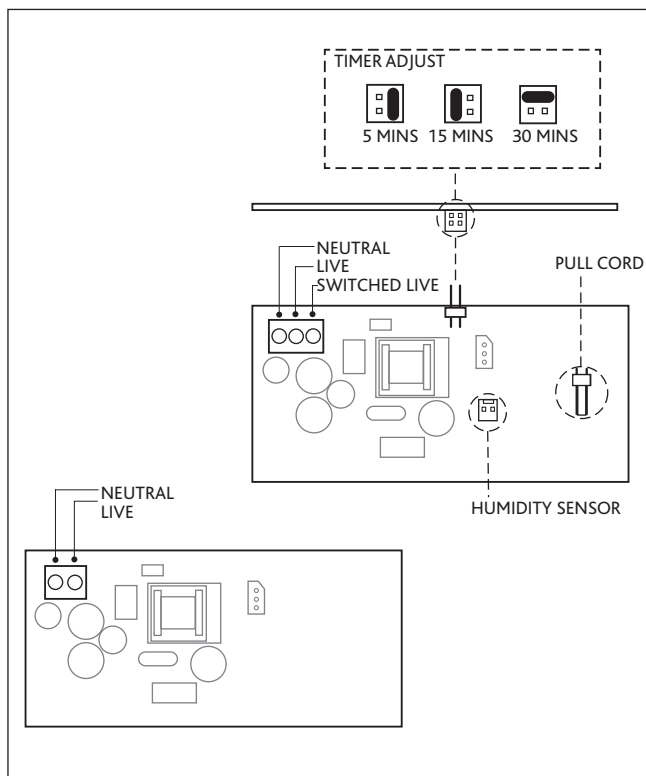
Figure 4d. Wiring. PCB details (where applicable)
